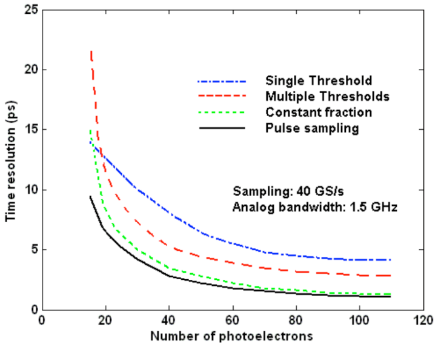
Figure 15 Electronics simulation of a CMOS multi-channel readout using various techniques. The analog bandwidth is 1.5 GHz, and an 8-bit ADC sampling at 40 GHz is used for the pulse sampling [23].
