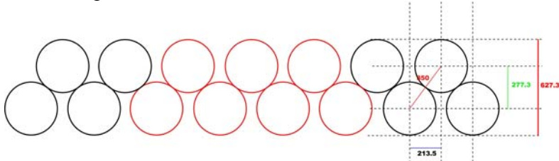
Figure 16 Arrangement of scintillating fibers in a tracker station plane as used in the MICE trackers). The fiber diameter is 350 \mu m, 7 fibers/channel, 1.63 mm/chan, which gives a resolution of 0.47 mm per plane. The fibers amount to 0.45% X_0 per double plane.
