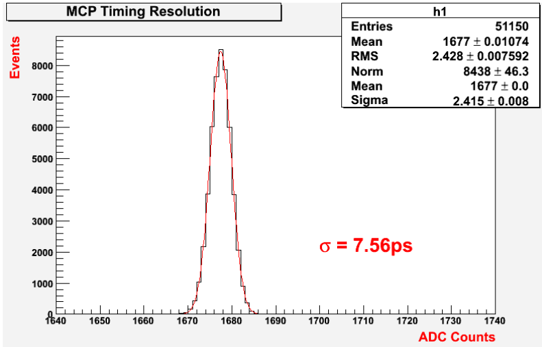
Figure 14 Measurement of the time difference between two commercial MCPs with 25 \mu m pores. Data are for a 408nm laser with ~50 photoelectrons, at the laser test stand at Argonne (Hamamatsu PLP-10 picosecond laser and a commercial CAMAC readout electronics system). The intrinsic jitter of the system is ~4ps and it has a resolution of 3.13ps [22]. The individual MCPs therefore have an intrinsic resolution about 4 ps.
