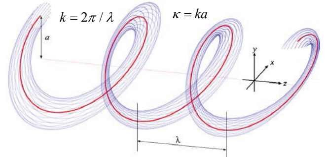
Figure 1: Schematic of beam motion in an HCC. Unlike cooling in a solenoid, the radius, a , does not diminish.
